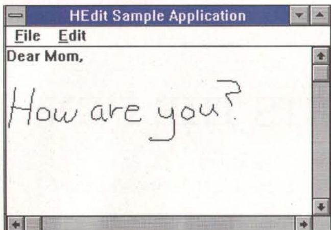
Screen 1: The PenPalette application converts the Edit control into an HEdit control, routes pen input through the handwriting recognizer, and feeds keystrokes into pen-oblivious applications.
